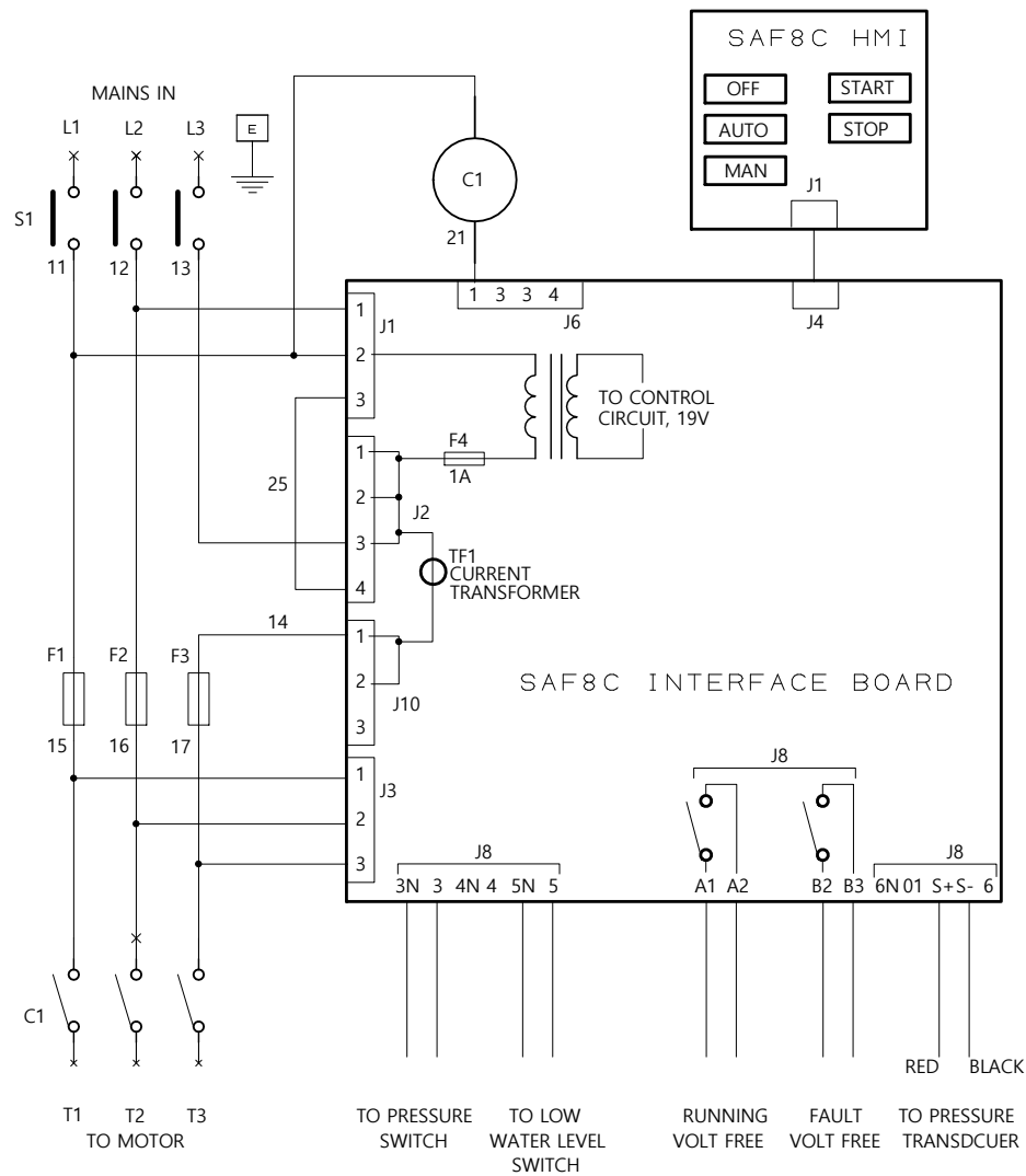
SCHEMATIC DIAGRAM
